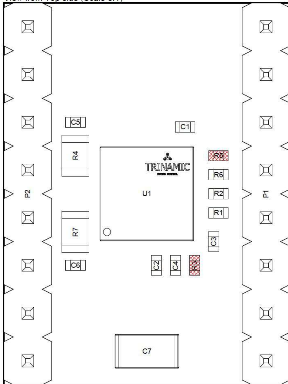
View from Top side (Scale 8:1)
